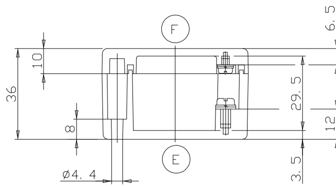
DECKEL
