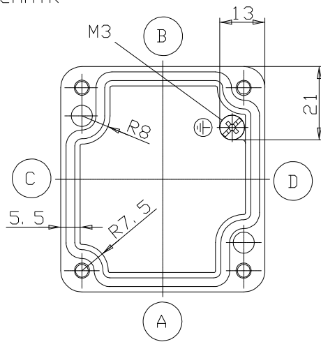
DECKEL
