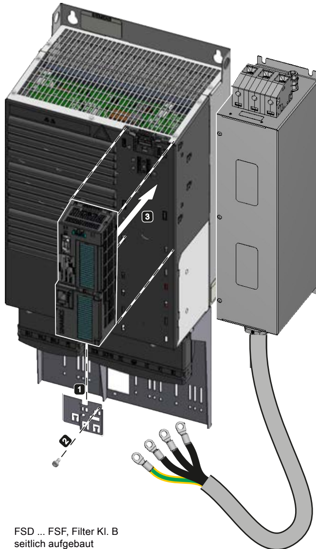
FSD .. FSF, Filter Cl. B, installed next to the inverter
